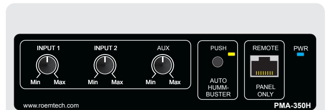
Front Panel
